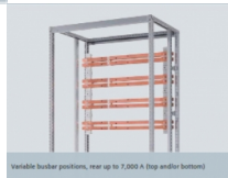
Variable busbar positions, rear up to 7,000 A (top and/or bottom)
